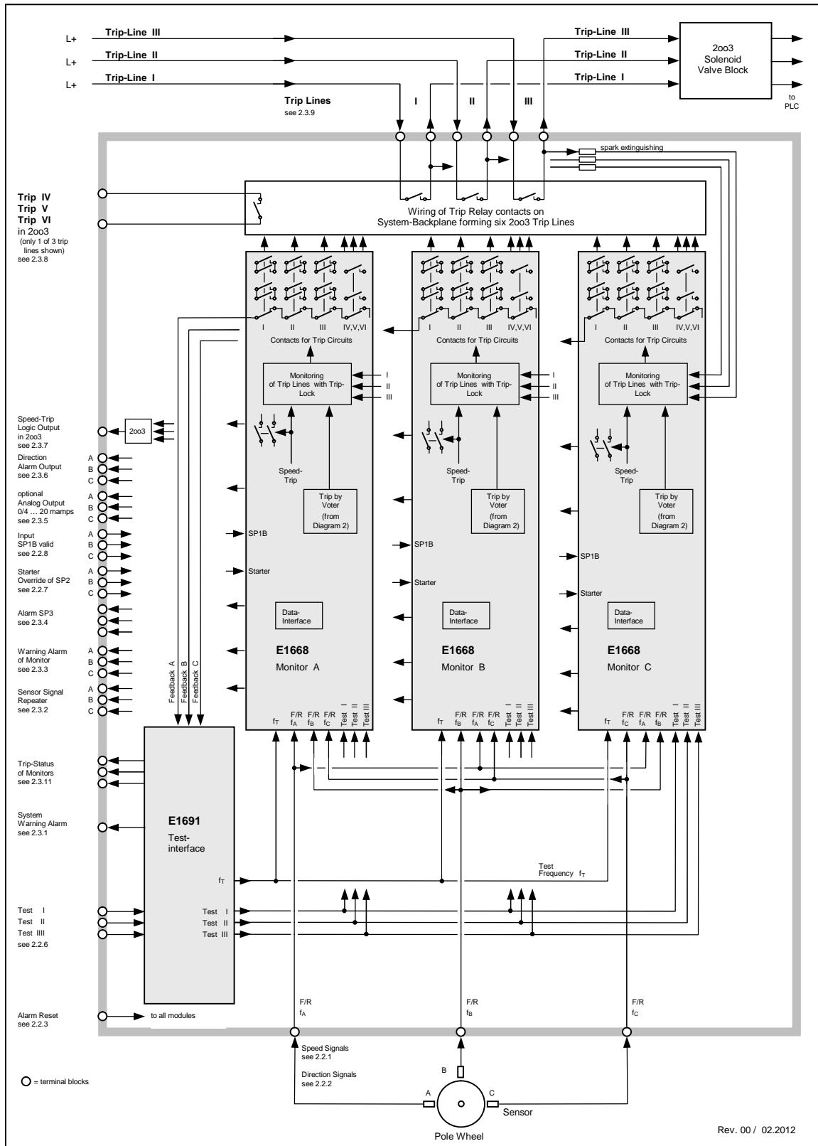
Figure 2: E16x352 System Structure Diagram 1 of 2
