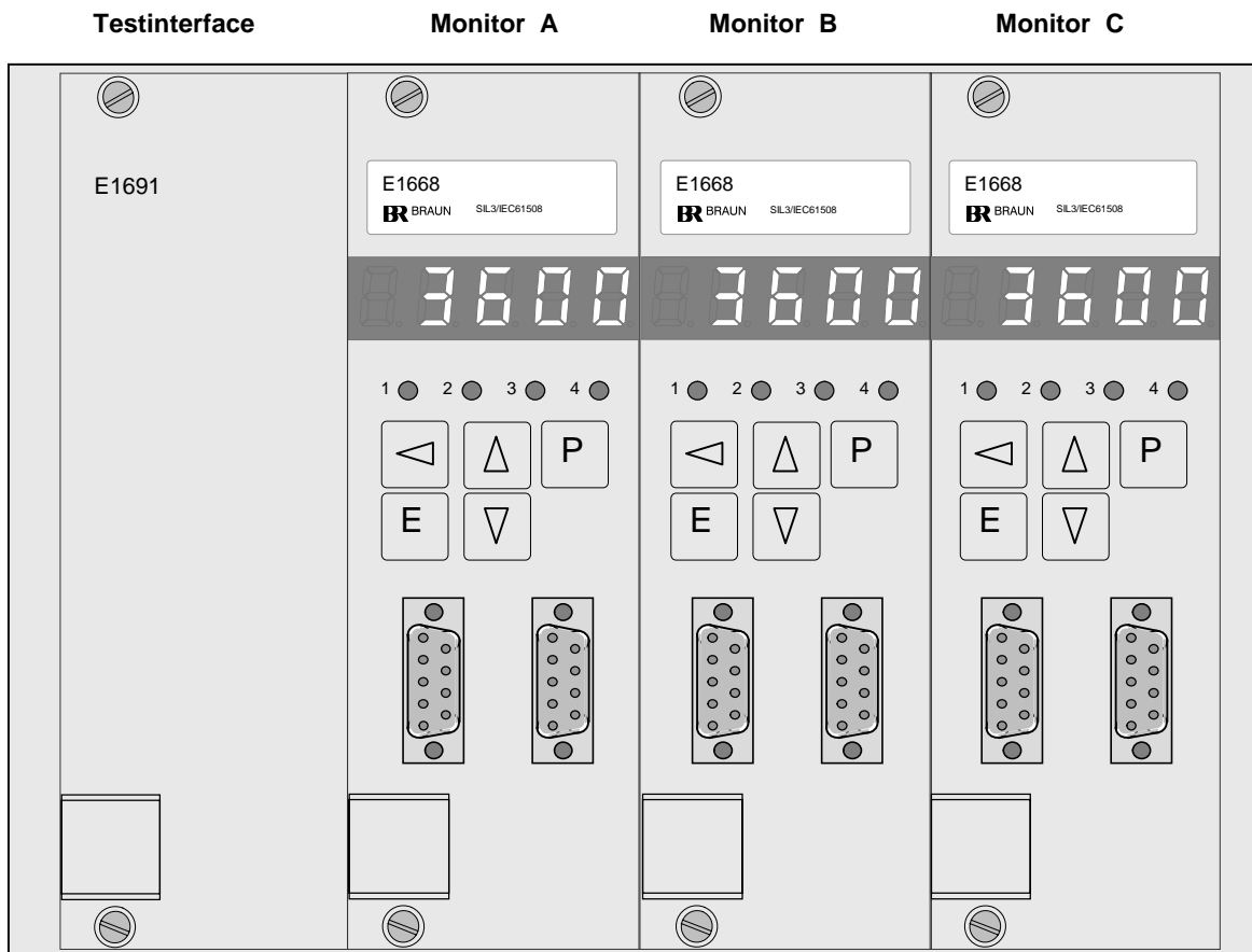
Figure 1: E16x352 System Front View
