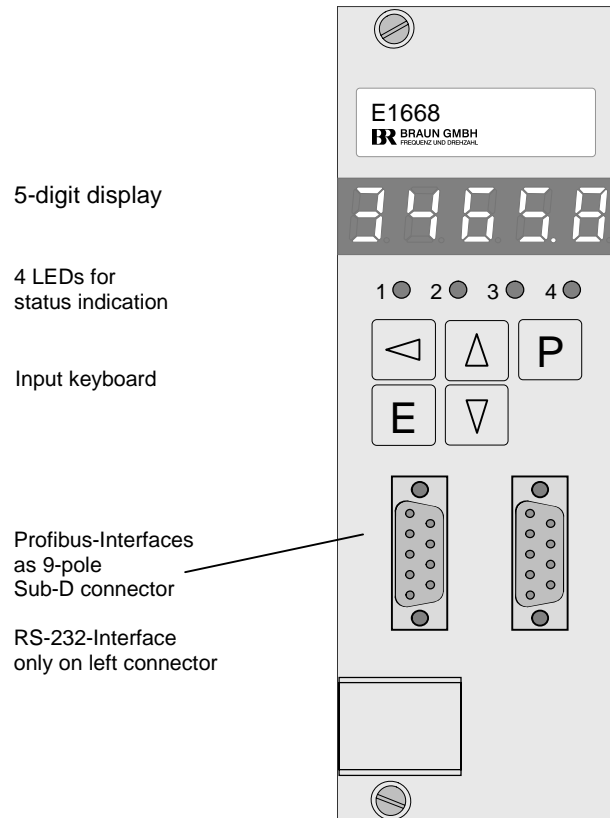
Figure 12: Front view of Monitor E1668
