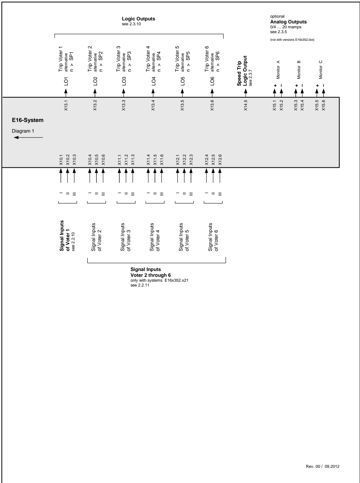
Figure 5: E16x352 System Wiring Diagram 2 of 3
