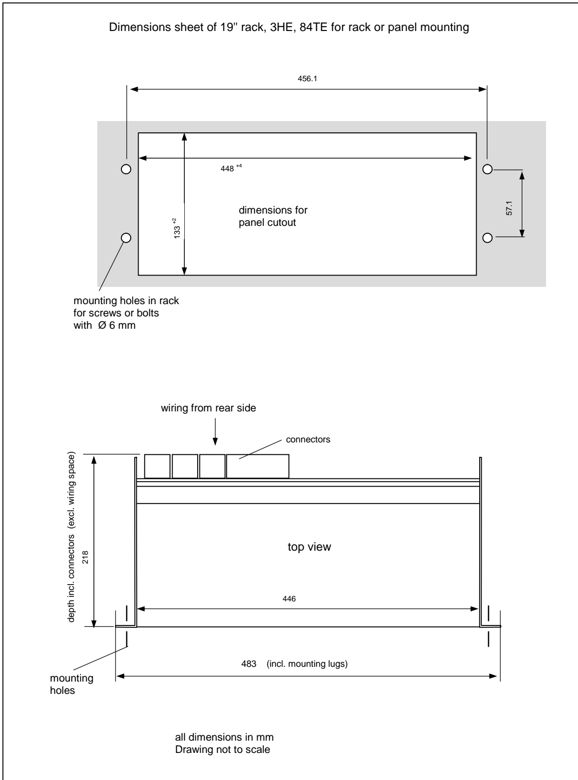
Figure 10: Dimensions of System E16E352
