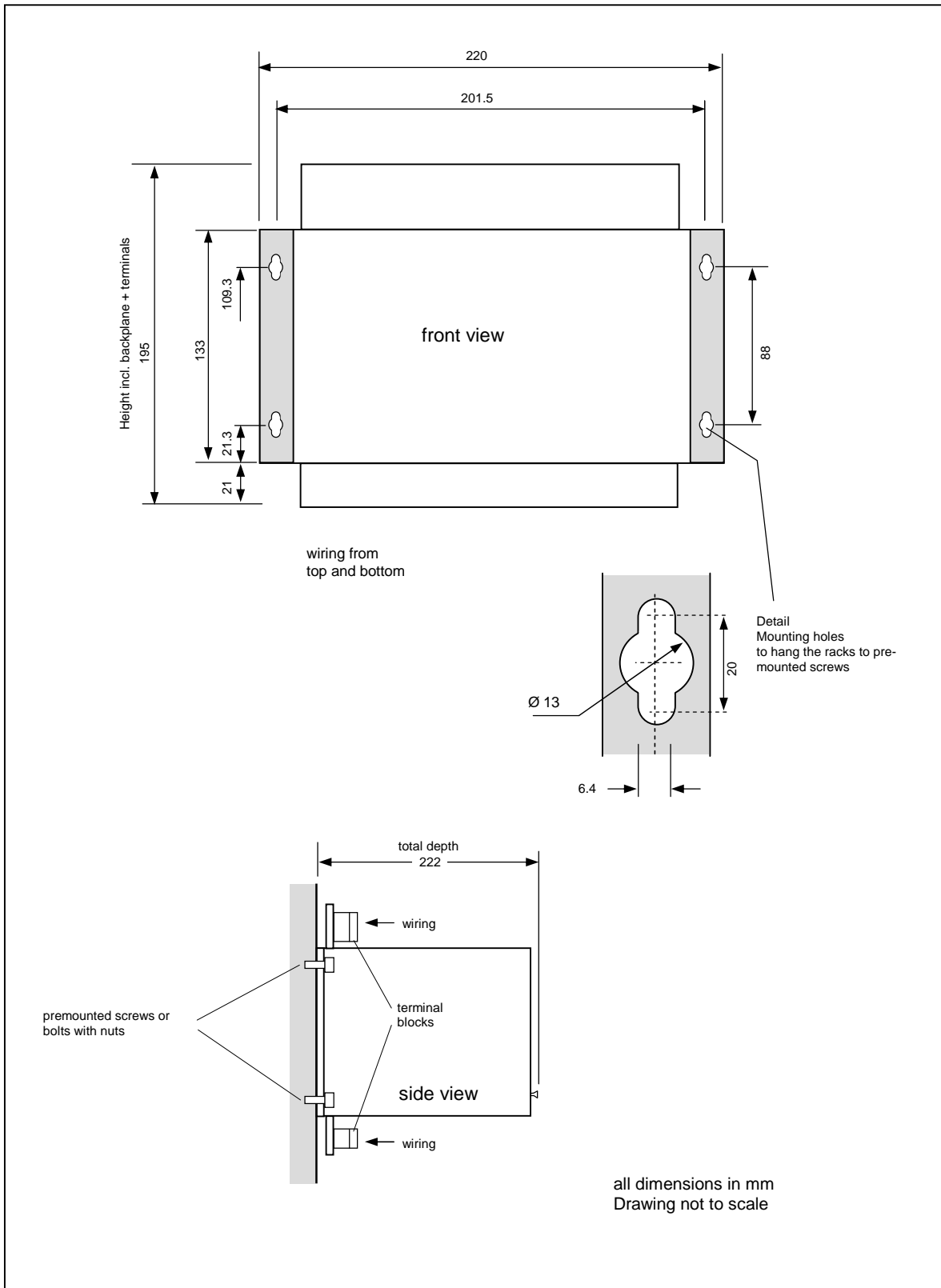
Figure 9: Dimensions of System E16A352
