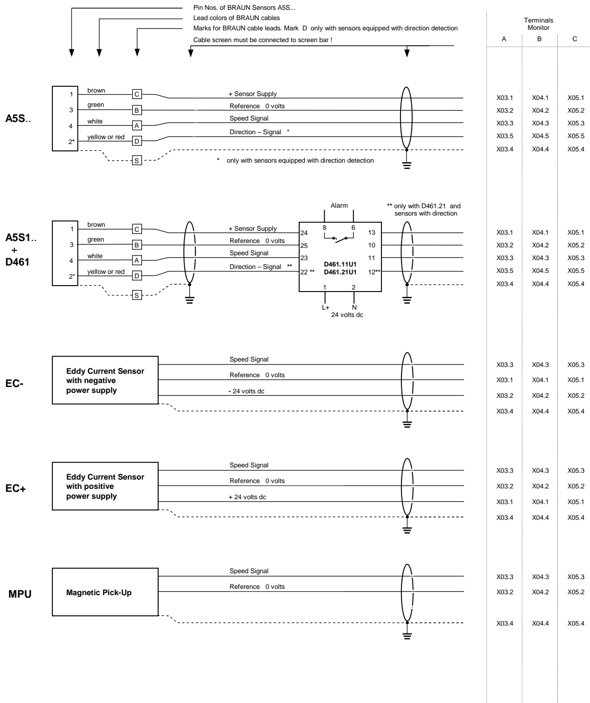
Figure 6: E16x352 System Wiring Diagram 3 of 3
